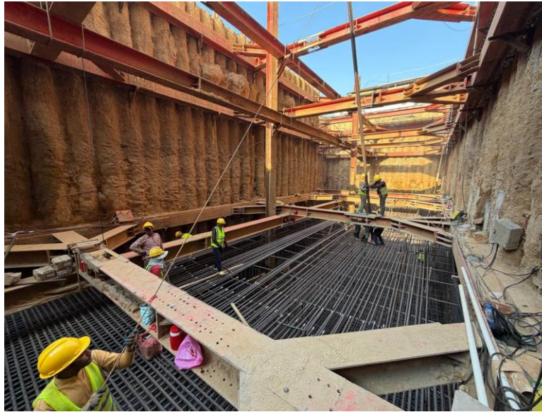
Installation of Top & Vertical bar of PC1
