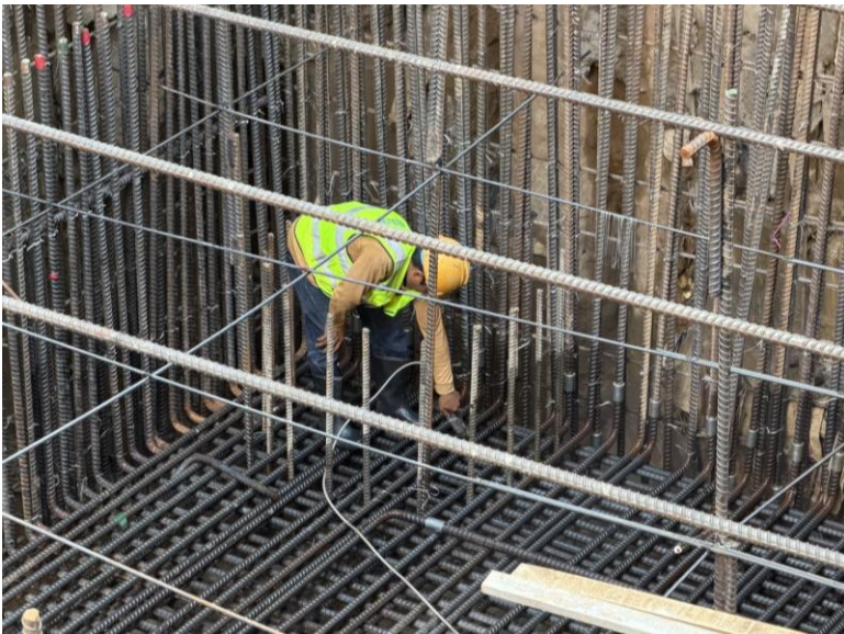
PC1 Bottom Bar cleaning
