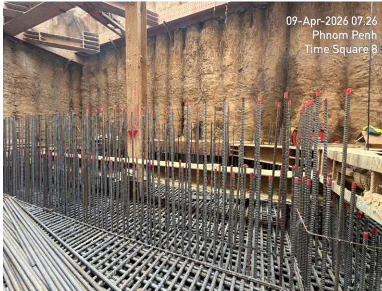
Inspection of Wall Starter Bars & Spacing
