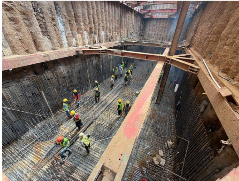
Installation of Bottom & Side bar of PC1
