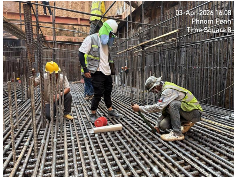
Inspection of Bottom & Side Bar
